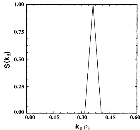
FIG. 8. k_\theta spectrum (in arbitrary units) of the potential in Fig. 6.
