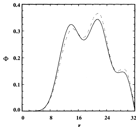
FIG. 10. Electrostatic potential (in arbitrary units) at \theta=0 vs minor radius (in units of \rho_i ) with the temperature profile effect retained (dotted line). The solid line represents the potential calculated without taking into account profile effect.
